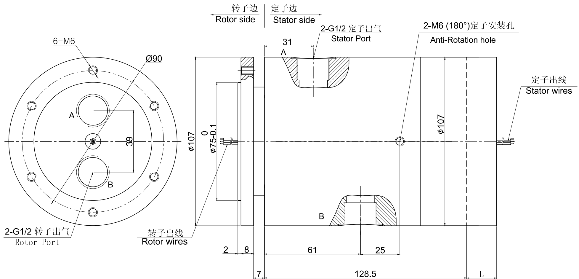
MAPH200S-05+Electricity size
